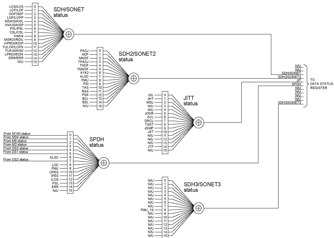
Figure 7-3 Status Registers Relationship 2
