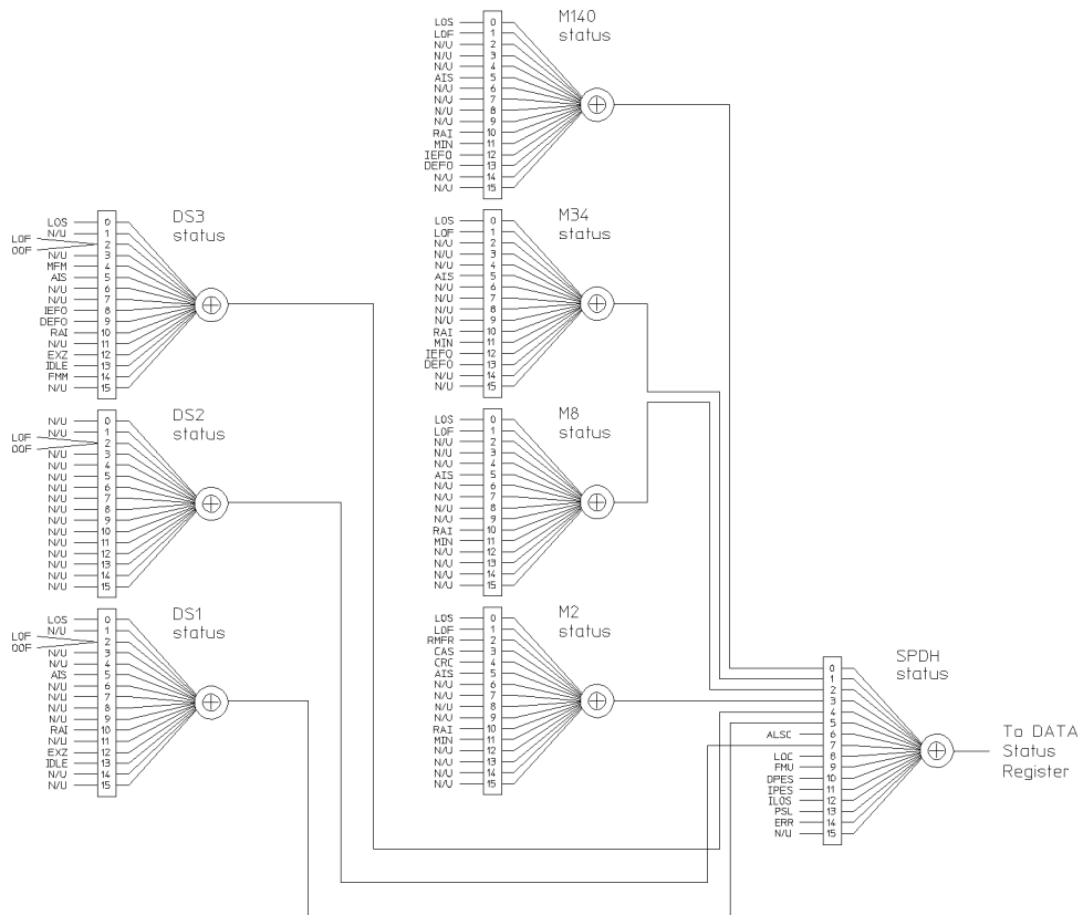
Figure 7-2 Status Registers Relationship 1
